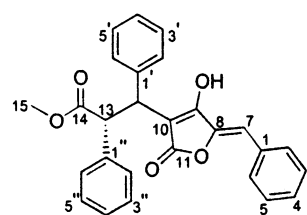
1 (12 R , 13 R ) and 2 (12 S , 13 R )
